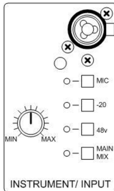
Figure 18: INSTRUMENT INPUT
