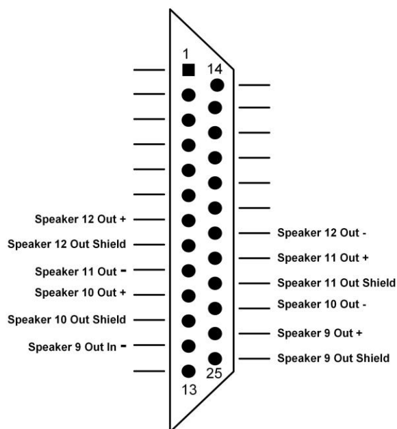
Monitor Speakers Outputs Pinout
