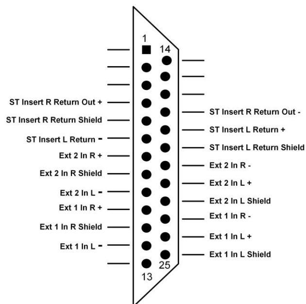
External Inputs / Stereo Insert Return
